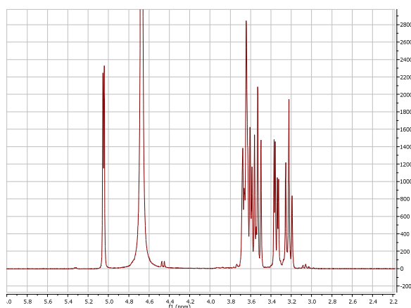
Glucose 1 H NMR spectrum in D 2 O at 300 MHz
