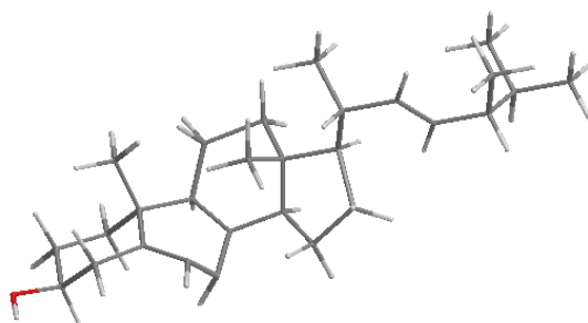
Ergosterol, ergosta-5,7,22-trien-3 \beta -ol, from Laetiporus sp.
